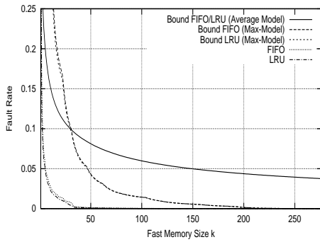
(c) SPARC, GCC, FIFO and LRU.
