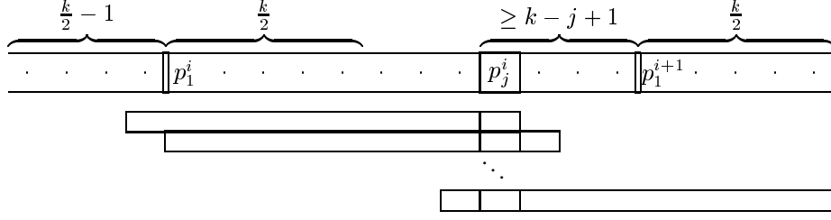
Figure 6: k even, j \geq \frac{k}{2} + 1 : p_j^i is contained in at least k - j + 1 + \frac{k}{2} windows contributing to N_k^i .
