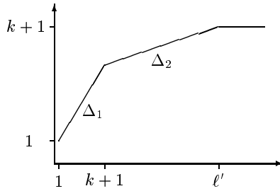
Figure 2: A(\ell) , an upper bound on \text{Av}(\ell) .
