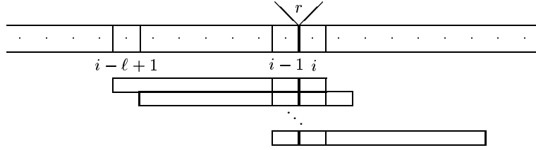
Figure 4: The windows \sigma_\ell[i - \ell + 1], \dots, \sigma_\ell[i - 1]
