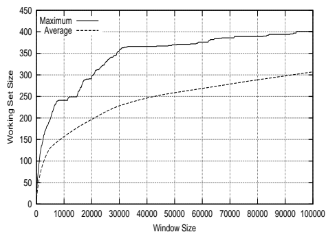
(a) VAX, PASCAL, 500 pages.
