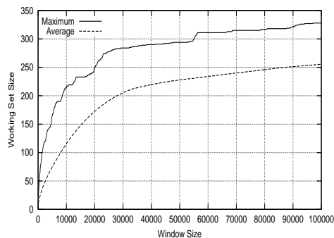
(b) VAX, SPIC, 385 pages.
