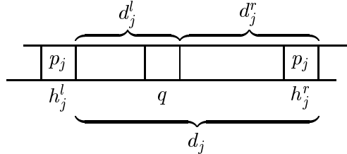
Figure 8: \sigma[h_j^l] : Last request to p_j before \sigma[q] . \sigma[h_j^r] : First request to p_j after \sigma[q] .
