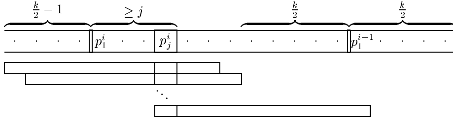
Figure 5: k even, j \leq \frac{k}{2} : p_j^i is contained in at least \frac{k}{2} - 1 + j windows contributing to N_k^i .
