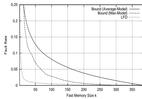
(b) VAX, SPIC, LFD
