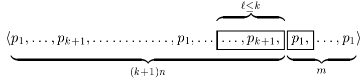
Figure 3: When \sigma_\ell[r(\ell)] is extended to \sigma_{\ell+1}[r(\ell)] , p_1 is included in the window.
