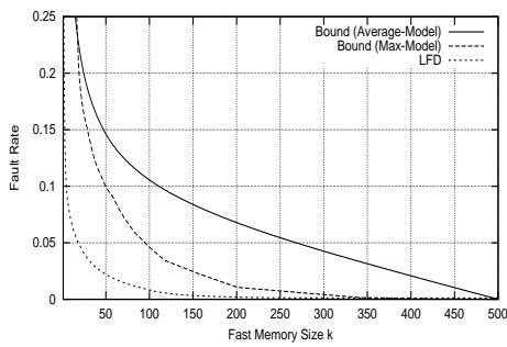
(a) VAX, PASCAL, LFD
