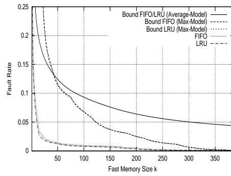
(b) VAX, SPIC, FIFO and LRU.
