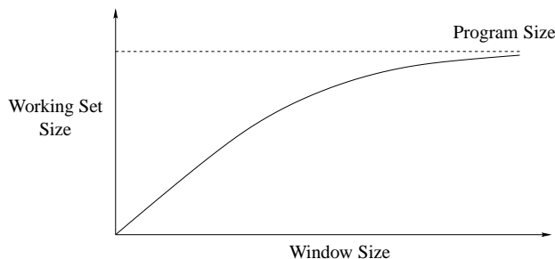
Figure 1: Working set size as a function of the window size.
