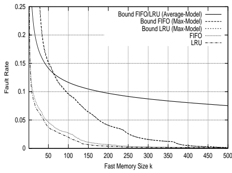
(a) VAX, PASCAL, FIFO and LRU.
